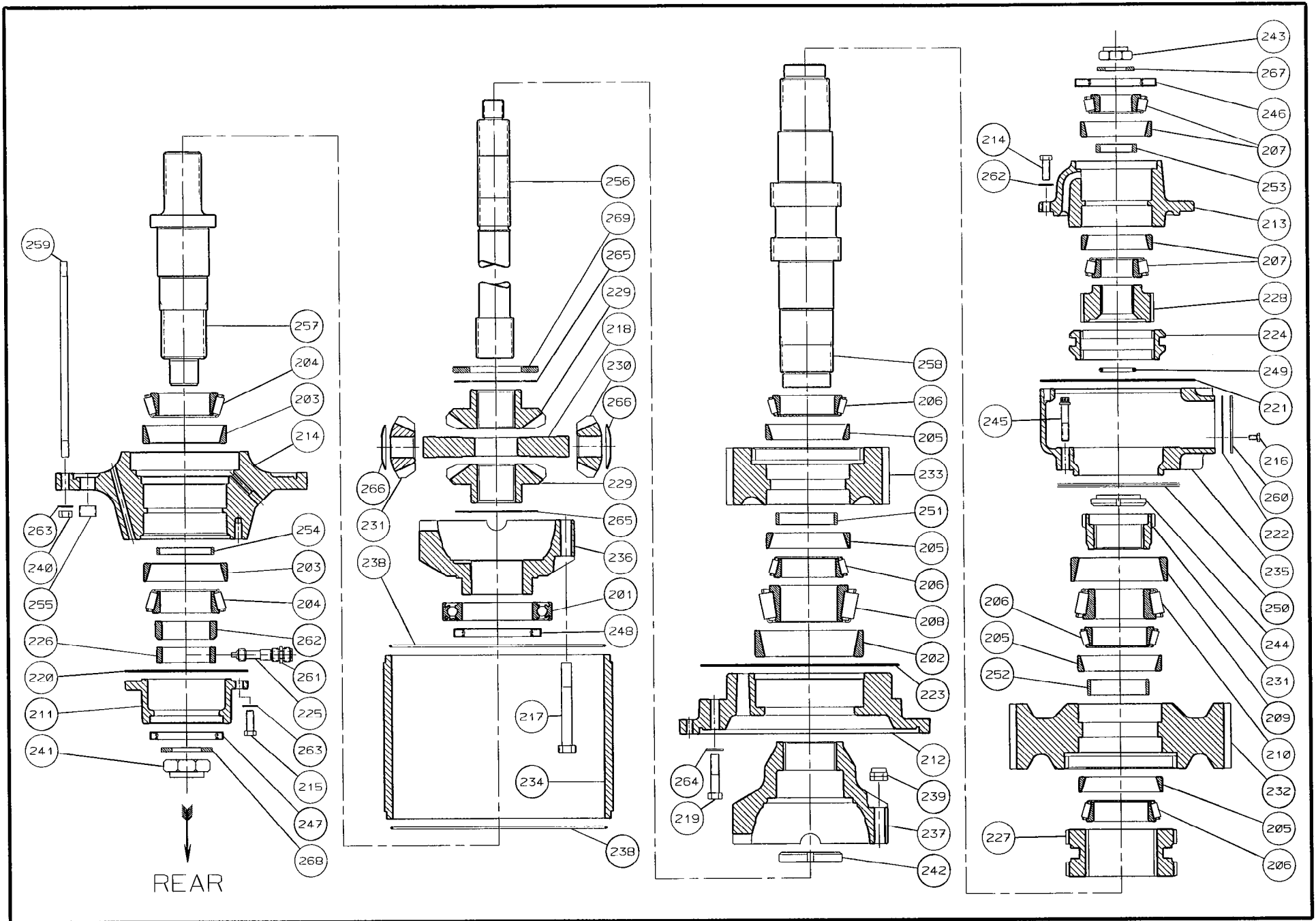
Pro Gear and Transmission • 906 W. Golf Blvd., Ft. Lauderdale, FL 33305, 1 (877) 742-6000 (409) 770-9001 FIGURE 8-1 TC 142PD 50/50 LOWER SHAFT PARTS
